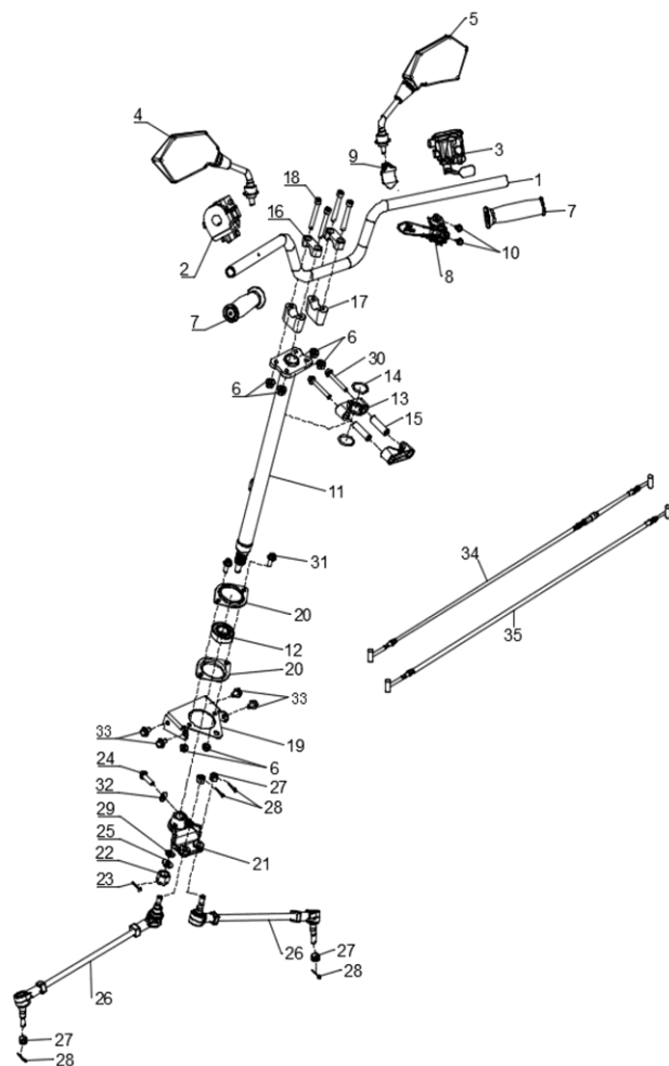
DIAGRAMMA 2025 MANUBRIO AODES F04
