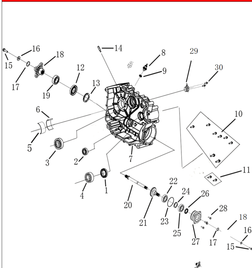
DIAGRAMMA 2025 CARTER DESTRO AODES E08
