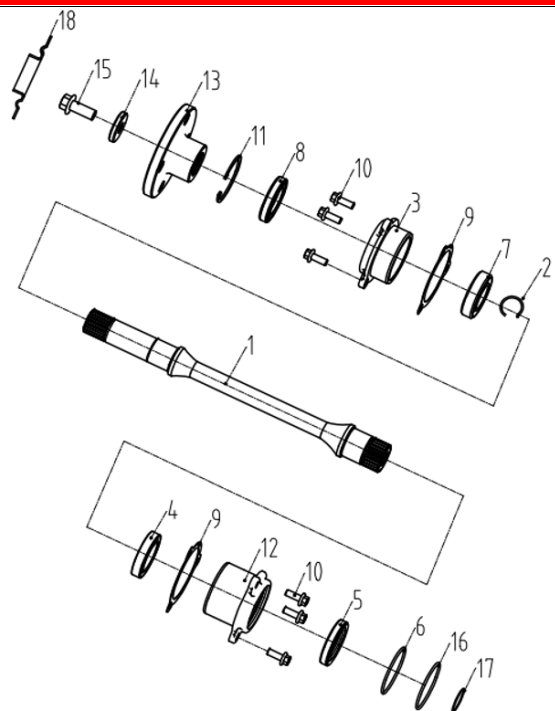
DIAGRAM 2025 AODES CVT TRANSMISSION E08
