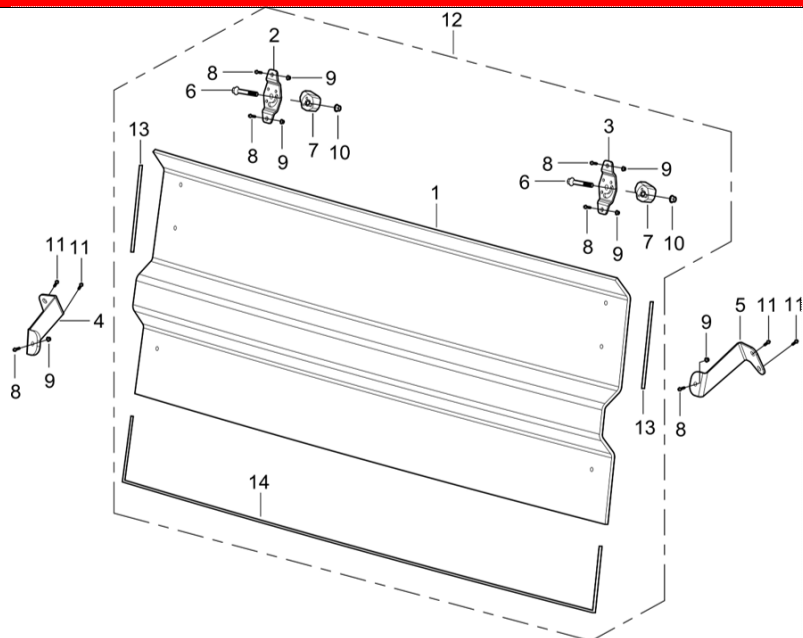
DIAGRAM 2025 AODES FRONT WINDSHIELD F29
